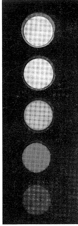
Fig. 7. The effect of ATP on the production of light by crystalline luciferase. All reagents were kept constant except for the ATP concentrations which were 0.08, 0.2, 0.4, 1.2, and 2.0 \cdot 10^{-4} M , increasing from left to right.
