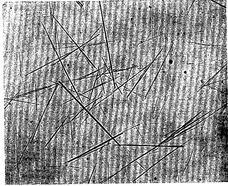
Fig. 1. Crystalline firefly luciferase. Magnification 100.
