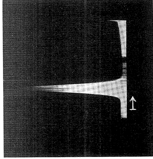
Fig. 2. Electrophoretic pattern of crystalline luciferase, pH 7.13 in 0.15\text{ M} NaCl and 0.02\text{ M} phosphate after 3 hours.
