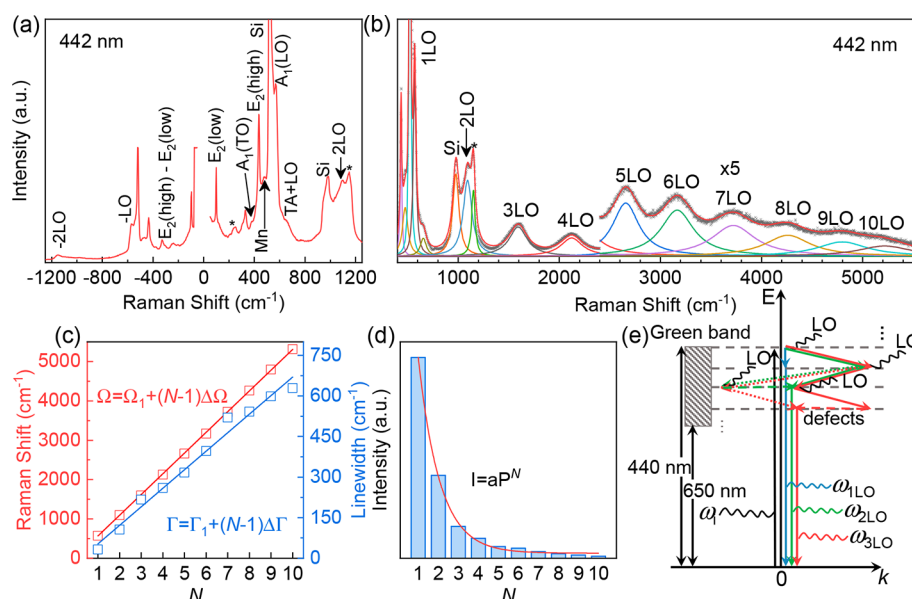
Figure 2. High-order phonon Raman scattering of Mn-doped ZnO NWs. (a) Raman spectrum of Mn-doped ZnO excited by a 442 nm laser. The stars mark unknown phonon modes. The corresponding higher wavenumber Raman spectrum with subtraction of the green band PL background is shown in part b. Lorentzian profiles are fitted to the LO phonon from N = 1 to 10 order. (c) Order number N dependence of the Raman shift \Omega and the linewidth \Gamma of the LO phonons. The solid lines denote linear fitting results. (d) Intensities of the NLO Raman modes as a function of N . The red line is the exponential fitting result. (e) Schematic diagram of the high-order Raman scattering. The black, blue, green, and red arrows represent the incident laser ( \omega_i ), 1LO, 2LO, and 3LO scattering processes, respectively. The dashed arrows denote the elastic scattering by the defects. The dotted arrows denote other possible scattering paths.
