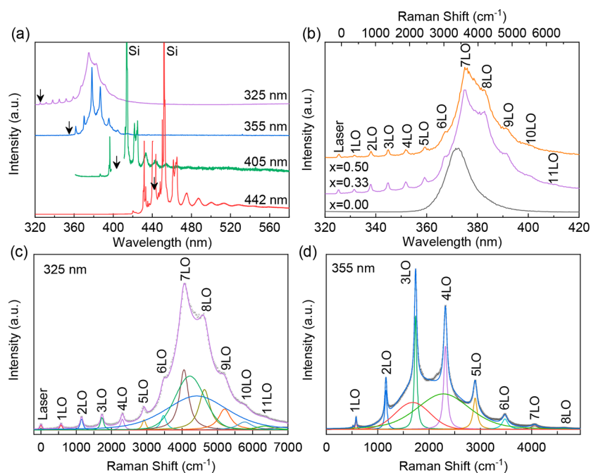
Figure 3. Hot luminescence spectra of Mn-doped ZnO NWs. (a) Spectra excited by different wavelength lasers. (b) Hot luminescence spectra of \text{Zn}_{1-x}\text{Mn}_x\text{O} ( x = 0.00, 0.33 , and 0.50 ) excited by a 325 nm laser. (c) 325 nm and (d) 355 nm excitation and the corresponding fitting results. The x -axis shows the relative frequency shift by offsetting the laser frequency to zero.
