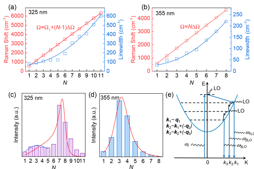
Figure 4. Cascade model of hot luminescence in Mn-doped ZnO NWs. Phonon peak frequency \Omega and the line width \Gamma extracted from spectra excited by (a) 325 nm and (b) 355 nm. The red and blue lines denote the linear fitting of the frequency and the parabolic fitting of the line width, respectively. Parts c and d are the fitted intensities from spectra excited by 325 and 355 nm, respectively. (e) Schematic diagram of the cascade model. Notice that k_1 , k_2 , and k_3 are the wave vectors of the photons with NLO phonon emissions and q_1 , q_2 , and q_3 are the phonon wave vectors.
