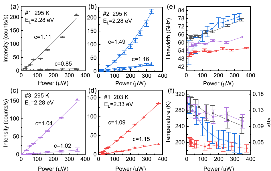
Figure 4. Power-dependent A'_1 mode intensity of Stokes (▲) and anti-Stokes (●) peaks of sample #1 (a), #2 (b), and #3 (c) at 295 K and #1 (d) at 203 K. Here, samples #1 and #2 are 3L WS 2 , and sample #3 is an hBN-encapsulated 3L WS 2 . The solid lines are fitted by the function of I = aP^c , where P is the power of excitation laser, and a and c are the fitting parameters. (e) The power-dependent linewidth of A'_1 phonon of different samples in (a–d). The error bar was evaluated by the temperature fluctuation of Si signal and instrument response.
