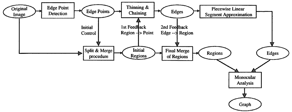
FIGURE 4. Scheme of the segmentation technique proposed by Bonnin et al. (1989). The edge information guides the split-and-merge procedure in both steps of the algorithm: first, to decide the split of a region, and second, in the final merging phase, to solve the possible oversegmentation.
