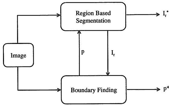
FIGURE 11. Flow diagram for game-theoretic integration of region-based segmentation and boundary finding proposed by Chakraborty and Duncan (1999). The outputs of each of the modules feed back to each other after every decision-making step. The algorithm stops when none of the modules can improve their positions unilaterally. (Reprinted from IEEE Transactions on Pattern Analysis and Machine Intelligence, vol. 21, no. 1, A. Chakraborty and J. S. Duncan, Game-Theoretic Integration for Image Segmentation , page 16, © 1999 IEEE.)
