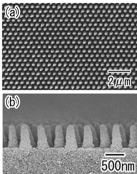
Figure 3. SEM images of TiO 2 pillar array: (a) surface and (b) cross-sectional view.
