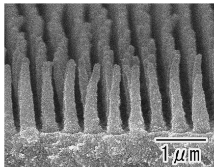
Figure 4. SEM image of TiO 2 pillar array with high aspect ratio.
