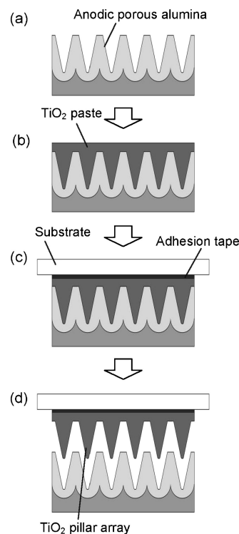
Figure 1. Schematic of fabrication process of TiO 2 nanopillar array: (a) anodic porous alumina mold with tapered holes, (b) filling of TiO 2 paste into alumina holes and heat treatment, (c) adhesion of substrate, (d) detachment of mold.
