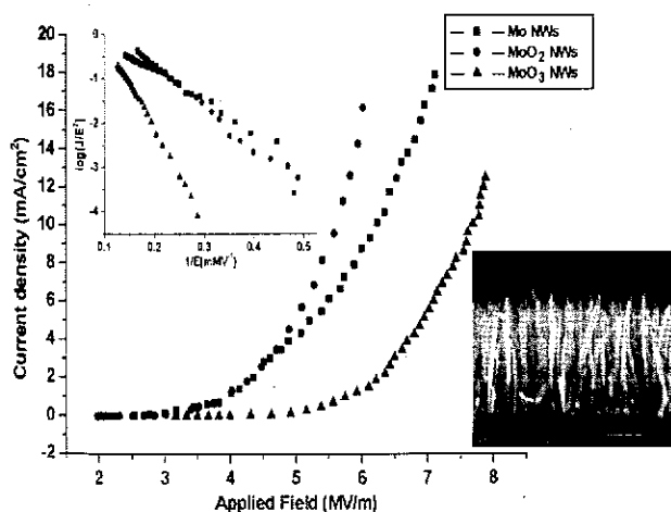
Fig. 20. Field emission current versus electric field ( I - E ) plots of the Mo, MoO 2 and MoO 3 nanowire arrays and their corresponding F-N plots (inset). The SEM image on right-hand side is aligned Mo nanowires (courtesy of Dr. Jun Zhou and Prof. N. S. Xue, Zhongshan University).
