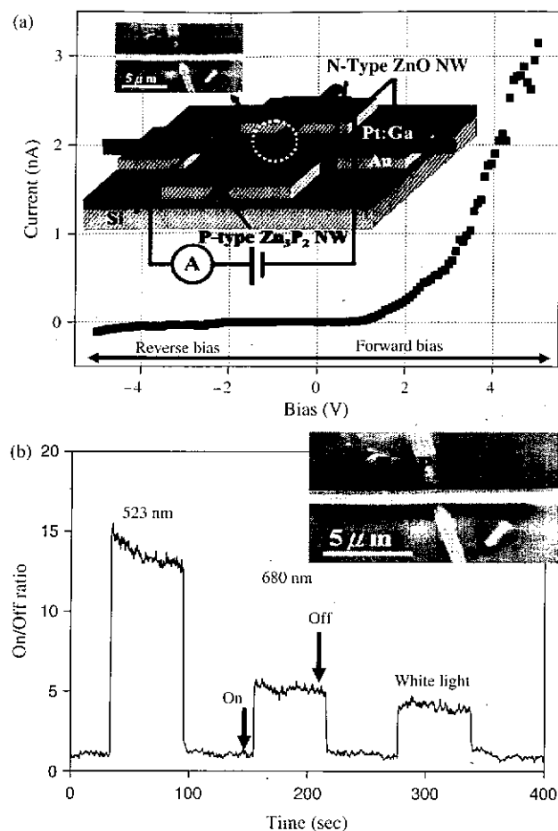
Fig. 26. (a) I - V curve for ZnO/ Zn_3P_2 nanoscale heterojunction at reverse and forward bias. Inset shows the prototype of the nanodevice, in which a ZnO NW was placed on top of a Zn_3P_2 NW. (b) The on/off ratio as a function of the time under red (680 nm), green (523 nm), or white light illumination, respectively. The inset is the schematic of the device. Reprinted with permission from [139], R. S. Yang et al., Nano Lett. 7, 269 (2007). © 2007, American Chemical Society.
