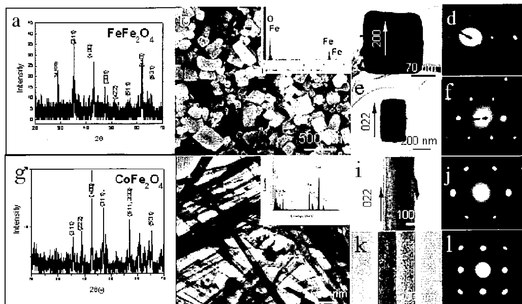
Fig. 16. Spinel (a–f) \text{Fe}_3\text{O}_4 nanoparticles and (g–l) \text{CoFe}_2\text{O}_4 nanobelts synthesized by the composite-hydroxide mediated approach. (a) XRD pattern of \text{Fe}_3\text{O}_4 ; (b) SEM image of \text{Fe}_3\text{O}_4 nanoparticles, and EDS pattern (insert). (c) A cube-like nanoparticle and (d) its electron diffraction pattern. (e) A \text{Fe}_3\text{O}_4 cuboids and (f) its diffraction pattern. (g) XRD pattern of \text{CoFe}_2\text{O}_4 nanobelts. (h) Morphology of the nanobelts and the corresponding EDS spectrum (insert) showing the presence of Co, Fe and O. The Si signal came from the TEM grid and holder. (i) A single-crystal nanobelt growing along [121] and (j) its electron diffraction pattern. (k) A nanobelt growing along [100] and (l) its electron diffraction pattern. Reprinted with permission from [109], H. Liu et al., Nano Lett. 6, 1535 (2006). © 2006, American Chemical Society.
