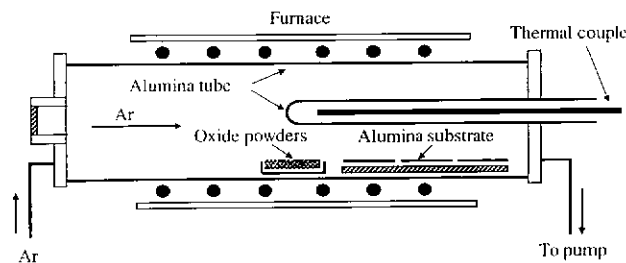
Fig. 2. Schematic diagram of experimental apparatus for growth of oxides nanostructures.
