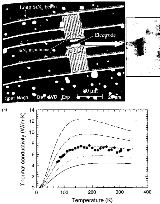
Fig. 22. (a) A microfabricated device for measuring the thermal conductivity of nanotubes, nanowires, and nanobelts. (b) Thermal conductivity of a 53 nm thick \text{SnO}_2 nanobelt as a function of temperature. Circles: measurement results; Lines: calculation results using the full dispersions transmission function approach with FL = 10.5 nm, 14.8 nm, 21 nm, 29.7 nm, and 42 nm, respectively for the five curves in the order of increasing thermal conductivity, where L is the characteristic length of the system. F is a parameter representing specularity of phonon reflection at the boundaries. Reprinted with permission from [131], L. Shi et al., Appl. Phys. Lett. 84, 2638 (2003). © 2003, American Institute of Physics.
