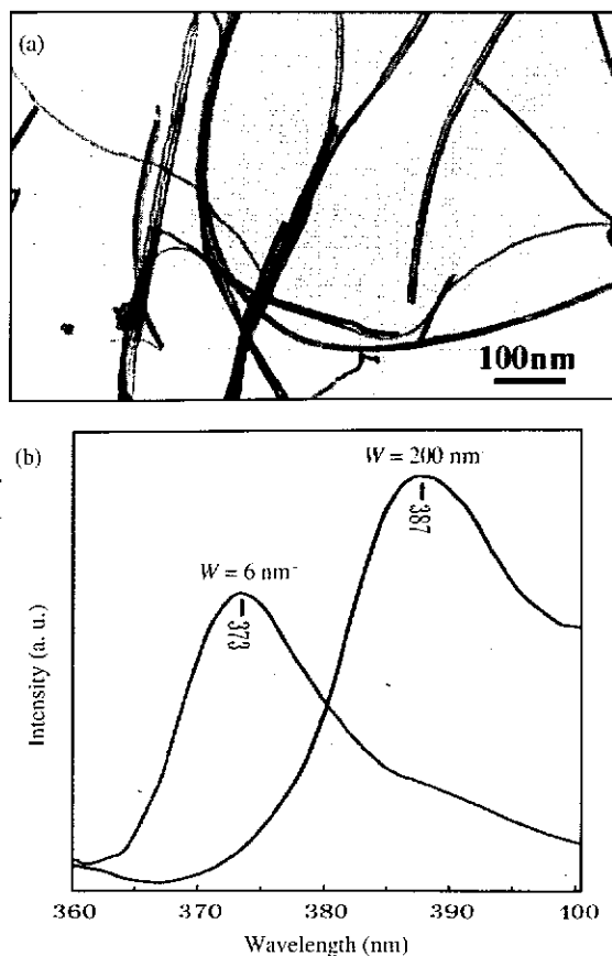
Fig. 25. (a) Low magnification TEM image showing the size uniformity of ZnO nanobelts. (b) Photoluminescence spectra acquired from the W = 200 \text{ nm} -wide ZnO nanobelts and the W = 6 \text{ nm} -wide ZnO nanobelts. Reprinted with permission from [136], X. D. Wang et al., J. Phys. Chem. B 108, 8773 (2004). © 2004, American Chemical Society.
