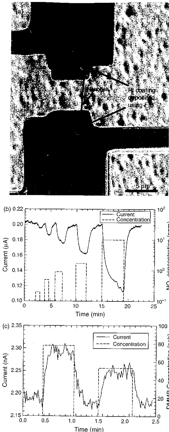
Fig. 23. Field effect transistor based gas sensors made using single nanobelt, and its application for detecting NO 2 DMMP. Reprinted with permission from [135], C. Yu et al., Appl. Phys. Lett. 86, 063101 (2005). © 2005. American Institute of Physics.
