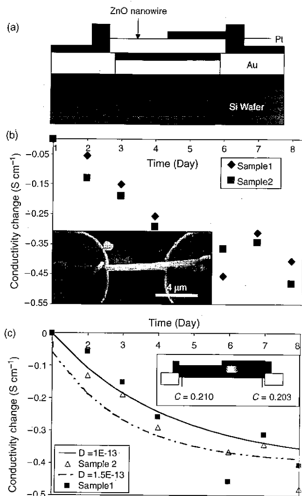
Fig. 24. (a) Schematic of ZnO nanowire placed on pre-patterned Au electrodes after Si 3 N 4 deposition. (b) Conductivity change of ZnO nanowires over time. The inset shows the SEM image of the device. (c) Illustration of curve fitting to determine the oxygen diffusion coefficient. The continuous lines represent the simulated results while the dots represent the experimental results. The inset shows simulated oxygen distribution on the eighth day after ion milling process.
