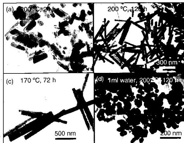
Fig. 15. TEM images of \text{BaMnO}_3 grown by the composite-hydroxide mediated approach at different time and temperature. (a) at 200 °C for 24 hours. (b) at 200 °C for 120 hours. (c) at 170 °C for 72 hours and (d) at 200 °C for 120 hours, adding 1 ml water. Reprinted with permission from [109], H. Liu et al., Nano Lett. 6, 1535 (2006). © 2006, American Chemical Society.
