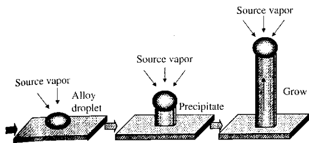
Fig. 1. Schematic diagram showing the growth of aligned nanowire arrays via the vapor-liquid-solid process.
