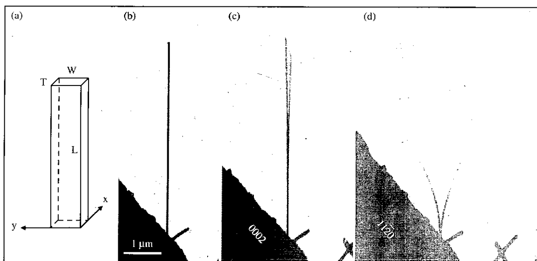
Fig. 17. Measuring the bending modulus of a nanobelt. (a) Geometrical shape of a nanobelt. (b) A ZnO nanobelt at stationary. (c, d) Mechanical resonance of the nanobelt along two orthogonal directions, respectively, closely perpendicular to the viewing direction ( \nu_x = 622 KHz), and nearly parallel to the viewing direction ( \nu_y = 691 KHz). Reprinted with permission from [117], X. D. Bai et al., Appl. Phys. Lett. , 82, 4806 (2003). © 2003, American Institute of Physics.
