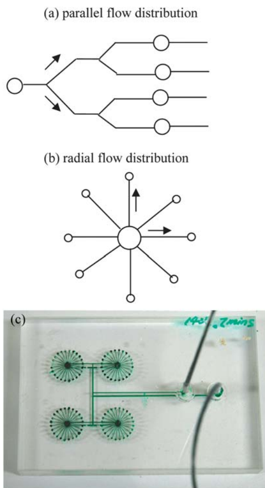
Fig. 1 Illustration of (a) parallel and (b) radial flow distribution and (c) a microfluidic device with radial flow distribution. The device is filled with a green food dye.
