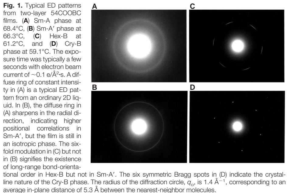
Fig. 1. Typical ED patterns from two-layer 54COOBC films. (A) Sm-A phase at 68.4°C, (B) Sm-A' phase at 66.3°C, (C) Hex-B at 61.2°C, and (D) Cry-B phase at 59.1°C. The exposure time was typically a few seconds with electron beam current of \sim 0.1 \text{ e}/\text{\AA}^2\cdot\text{s} . A diffuse ring of constant intensity in (A) is a typical ED pattern from an ordinary 2D liquid. In (B), the diffuse ring in (A) sharpens in the radial direction, indicating higher positional correlations in Sm-A', but the film is still in an isotropic phase. The six-fold modulation in (C) but not in (B) signifies the existence of long-range bond-orientational order in Hex-B but not in Sm-A'. The six symmetric Bragg spots in (D) indicate the crystal-line nature of the Cry-B phase. The radius of the diffraction circle, q_0 , is 1.4 \text{ \AA}^{-1} , corresponding to an average in-plane distance of 5.3 \text{\AA} between the nearest-neighbor molecules.
