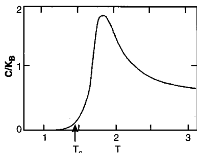
Fig. 4. Theoretical prediction of the C_p profile for a KT-type transition in two dimensions (27). The heat capacity should involve only an essential singularity at the transition temperature T_c that is not expected to be observable, as well as a broad hump far above T_c due to the gradual dissociation of defect pairs—for example, dislocation pairs in the crystalline phase and disclination pairs in the hexatic phase.
