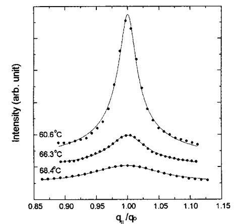
Fig. 3. Radial q_{\parallel} scans from a two-layer 54COOBC film at 68.4°C (Sm-A), 66.3°C (Sm-A'), and 60.6°C (Hex-B phase). The corresponding positional correlation lengths are 14.5 \pm 0.6 , 33.1 \pm 1.3 , and 76.5 \pm 4.0 \text{ \AA} , respectively. The points are data and the solid lines are Lorentzian fits in the Sm-A and square-root Lorentzian fits in the Sm-A' and Hex-B phase. The abscissa is normalized to the peak position, q_0 , of the radial line shape.
