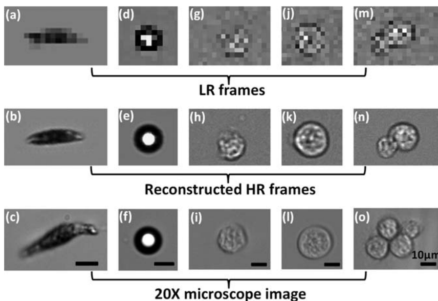
Fig. 2 Images obtained from the SROFM device. Euglena gracilis (a–c), microsphere (d–f) and Entamoeba invadens cysts (g–o). Raw low resolution (LR) images from the sensor (top row), high resolution (HR) images reconstructed from the sequence of LR images (middle row) and conventional bright field microscope images taken with 20x objective lens (bottom row). 40 to 50 LR frames were used to reconstruct each HR image.
