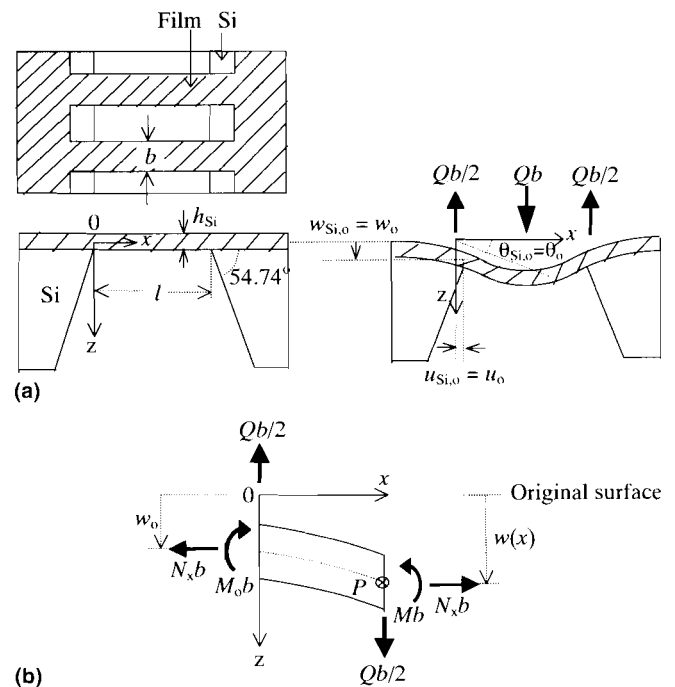
FIG. 1. (a) Schematic presentation of the configuration of a single-layered silicon nitride microbridge and the coordination system. (b) Moments and forces acting on a segment.
