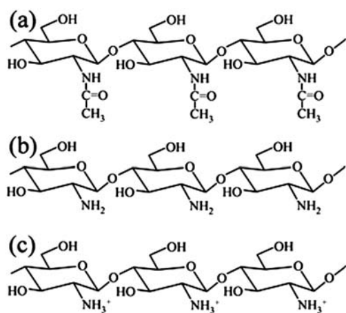
Fig. 1 Structural formulas of chitin and chitosan showing the three possible states of the amine group: (a) chitin, amine group acetylated; (b) chitosan, amine group free; (c) chitosan, amine group protonated.
