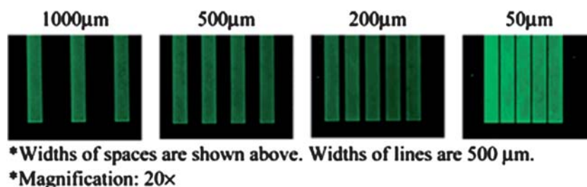
Fig. 5 Resolution of spaces between 500 \mu\text{m} wide gold lines after chitosan deposition and subsequent reaction with NHS fluorescein. The widths of spaces were 1000, 500, 200, and 50 \mu\text{m} . Reprinted with permission from ref. 12. Copyright 2003 American Chemical Society.
