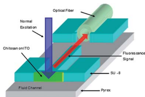
Fig. 11 Perspective view of optical waveguide sensor with chitosan film on sidewall. The waveguide is shortened to show fiber coupling. The blue arrow represents the optical excitation signal while the red arrow represents the collected fluorescence signal. 20 —Reproduced by permission of the Royal Society of Chemistry.
