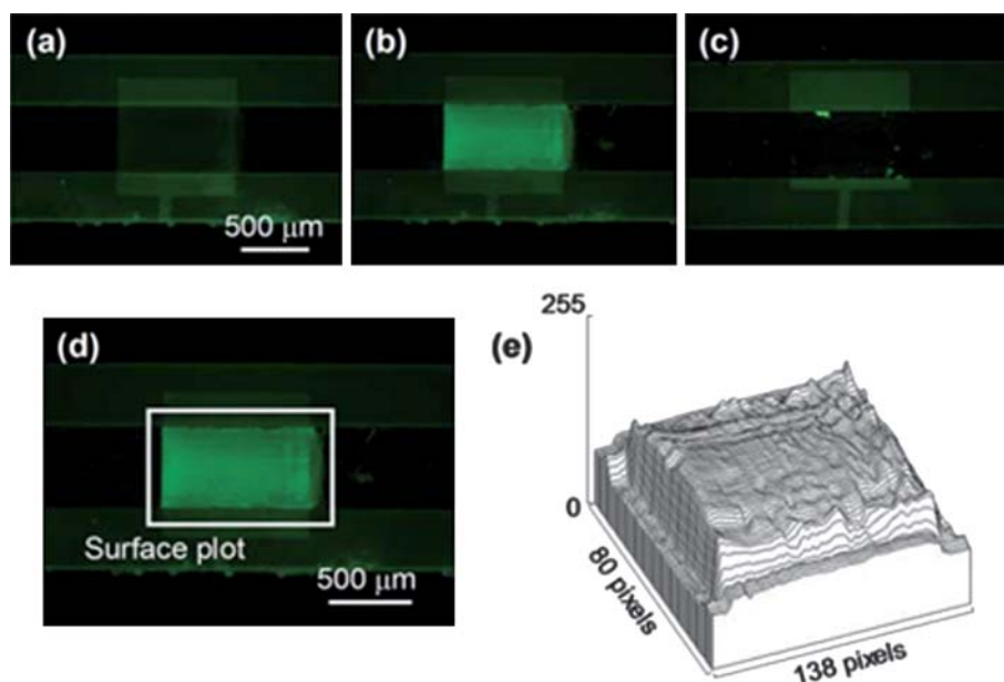
Fig. 7 Chitosan mediated assembly of GFP in micro fluidic device. (a) Fluorescence image of the assembly site after glutaraldehyde reaction; (b) after GFP reaction; (c) negative control (no bias); (d) GFP conjugated chitosan film; (e) Image J fluorescence surface plot. 57 —Reproduced by permission of the Royal Society of Chemistry.
