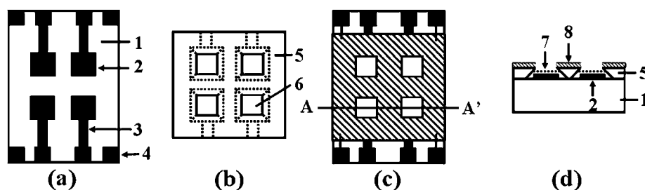
Fig. 10 Schematic of micromachined amperometric sensor. 1. Pyrex glass down-substrate, 2. Pt WE, 3. Conduction line, 4. Pads, 5. Up-substrate made of silicon, 6. Quadratic hole, 7. Chitosan membrane with cross-linked enzyme, 8. Ag/AgCl RE. (a) Down-substrate, (b) up-substrate, (c) bonding between up- and down-substrates, (d) cross section along A-A'. Redrawn with permission from ref. 24.
