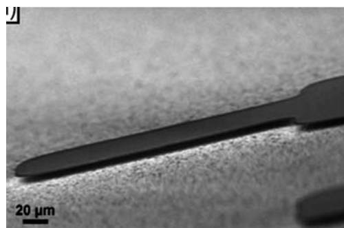
Fig. 14 Partially released chitosan cantilever on silicon with dimensions 240 \times 25 \times 2 \mu\text{m} . Chitosan serves as a sufficient structural material to support itself. Reprinted with permission from ref. 14. © 2008 IEEE.
