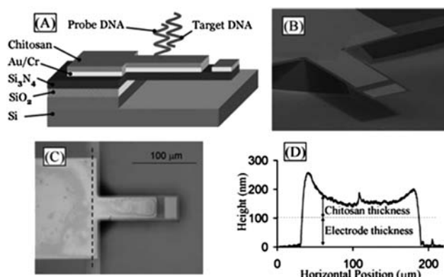
Fig. 13 (a) Schematic of microcantilever with chitosan used for detection of DNA hybridization and for detection of dopamine electrochemical oxidation. (b) SEM of fabricated cantilever. (c) Optical micrograph of cantilever after chitosan electrodeposition. The chitosan is deposited everywhere except at the electrically isolated tip. (d) Contact profiler scan of chitosan film along dashed line in C. 27 —Reproduced by permission of the Royal Society of Chemistry.
