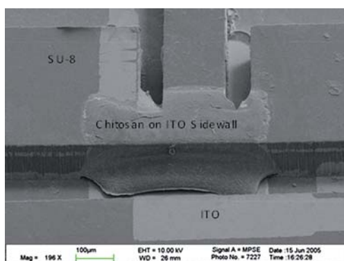
Fig. 4 SEM of chitosan film electrodeposited on the sidewall of a microchannel. A thin film of patterned indium tin oxide acted as the cathode surface for the deposition. Reprinted with permission from ref. 162.
