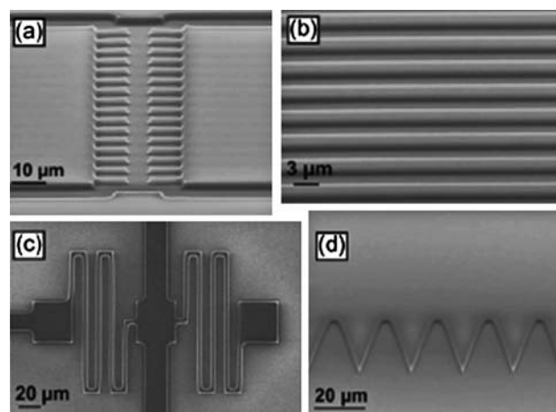
Fig. 2 Photolithographically patterned chitosan features. (a) SEM of matched comb structure at a 50° tilt. (b) SEM of 2- \mu m-wide lines with 4- \mu m pitch. (c) SEM of serpentine spring structures. (d) SEM of a sawtooth structure. Note: All patterns are in a 2- \mu m-thick chitosan layer. Reprinted with permission from ref. 14. © 2008 IEEE.
