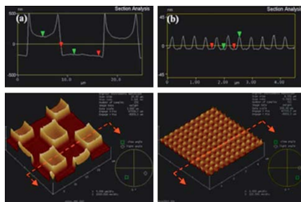
Fig. 6 Examples of AFM images taken of (a) printed chitosan squares 6.7\ \mu\text{m} across and (b) chitosan nanodots with 150\ \text{nm} width and 400\ \text{nm} pitch. Reprinted with permission from ref. 13. Copyright 2007, American Institute of Physics.
