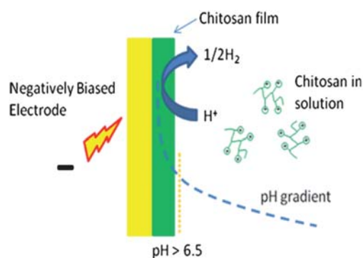
Fig. 3 Schematic demonstrating chitosan film electrodeposition. Adapted with permission from ref. 6. Copyright 2005 American Chemical Society.
