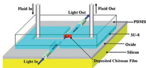
Fig. 12 Schematic of the microfluidic sensor for phenol detection. Both waveguides patterned perpendicular to the channel allow for in-plane light interrogation. Reprinted from ref. 54 with permission from Elsevier.
