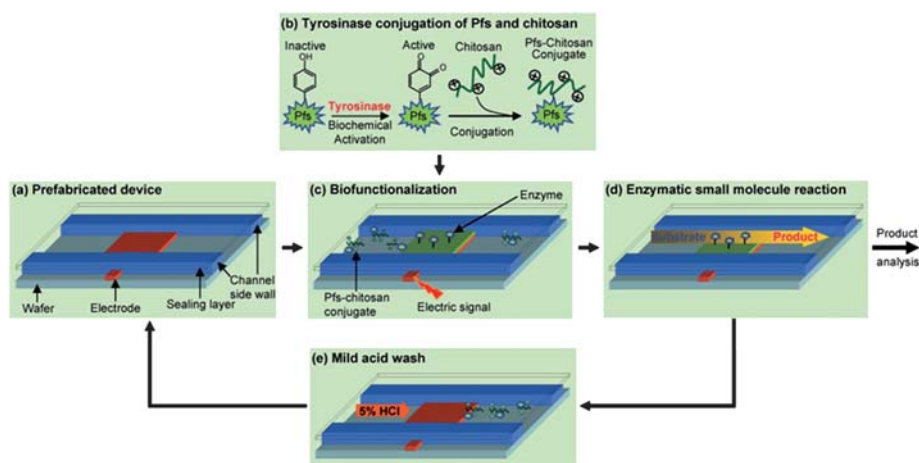
Fig. 8 Schematic of chitosan conjugation and electrodeposition in a microfluidic channel. (a) Prefabricated device, (b) conjugation between chitosan and the enzyme Pfs, (c) electrodeposition of Pfs-chitosan conjugate, (d) enzymatic small molecule detection, (e) mild acid wash removes chitosan and refreshes electrode surface. 58 —Reproduced by permission of the Royal Society of Chemistry.
