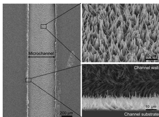
Fig. 2 SEM images of vertically aligned FF peptide NWs within the microchannel. The microchannel (500 μm width × 50 μm height × 3 cm length) was fabricated using polyvinylsilazane through soft-lithographic process, and the peptide/Pd NWs were subsequently grown on both bottom and sidewalls of the channels by self-assembly.
