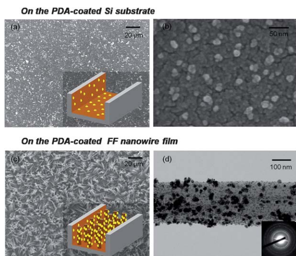
Fig. 3 (a and b) SEM images of Pd nanoparticles on PDA-coated Si substrate with different magnifications, (c) SEM and (d) TEM images of Pd nanoparticles on the PDA-coated FF peptide nanowire film. The loaded amount of Pd nanoparticles on the FF peptide NWs is much larger than that of the flat substrate due to highly increased surface area. The SAED pattern on (d) shows polycrystalline diffraction rings corresponding to fcc Pd.
