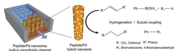
Fig. 1 Scheme for peptide/Pd nanowires built-in microfluidic system for heterogeneous catalytic hydrogenation and Suzuki coupling reactions.
