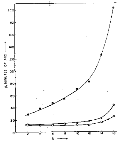
FIGURE 6. The line breadths \beta_x for the wolfram spectra plotted against N . \circ from the sample annealed at 1300^\circ\text{C} ; \bullet from the sample recovered at 1150^\circ\text{C} ; \bullet from the sample examined as filed; \blacktriangle subsidiary measurement of aluminium line 24.
