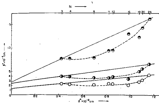
FIGURE 5. The interpretation of the line broadening in the aluminium spectra in which \beta^* is plotted against d^* assuming an experimental breadth of 12 mins. of arc. Symbols as for Figure 4.
