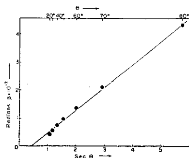
FIGURE 2. A plot of the physical broadening \beta due to simultaneous small particle size and strain broadening against \sec \theta . Any reasonable line through the calculated points gives a negative intercept.
