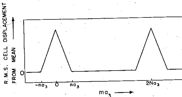
FIGURE 11. Schematic representation of the variation of the root mean square displacement of the cells with distance in recovered metals.
