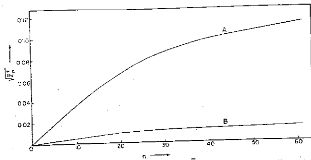
FIGURE 10. The variation of \sqrt{Z_n^2} with n for line 14 wolfram. The curves have been fitted to the experimental points at the same values of n as in Figure 8. A from the as filed sample; B from the sample recovered at 1150°C.
