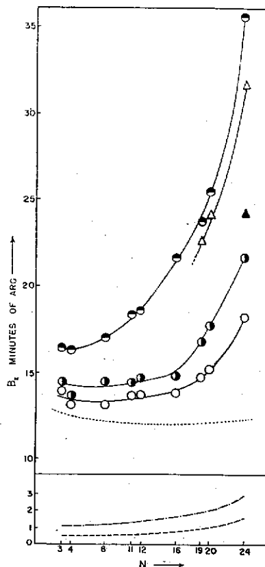
FIGURE 4. The line breadths \beta_{\chi} for the aluminium spectra plotted against N = h^2 + k^2 + l^2 . \circ from the high purity annealed sample; \bullet from the high purity filed sample; \bullet from the commercial purity filed sample; \Delta from the slowly mechanically filed high purity sample; \blacktriangle from the high purity samples rapidly filed under liquid air; \dots the predicted form of the experimental broadening; --- physical broadening produced by a particle size of 10^{-4} cm; - \cdot - \cdot - physical broadening produced by a particle size of 5 \times 10^{-5} cm.
