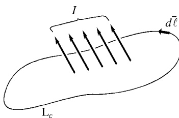
Figure 4.7 Loop L_c encloses current I . The line integral of the H or B field around the loop in the direction shown by vector d\vec{\ell} is proportional to I .
