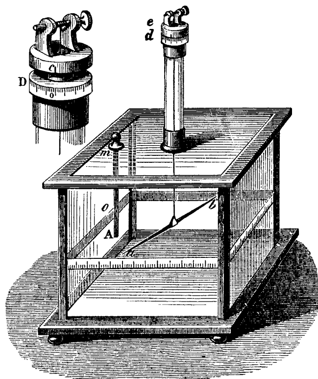
Figure 2.3 This is a diagram of the sort of torsion balance used to verify Coulomb's law for the poles of a permanent magnet.
