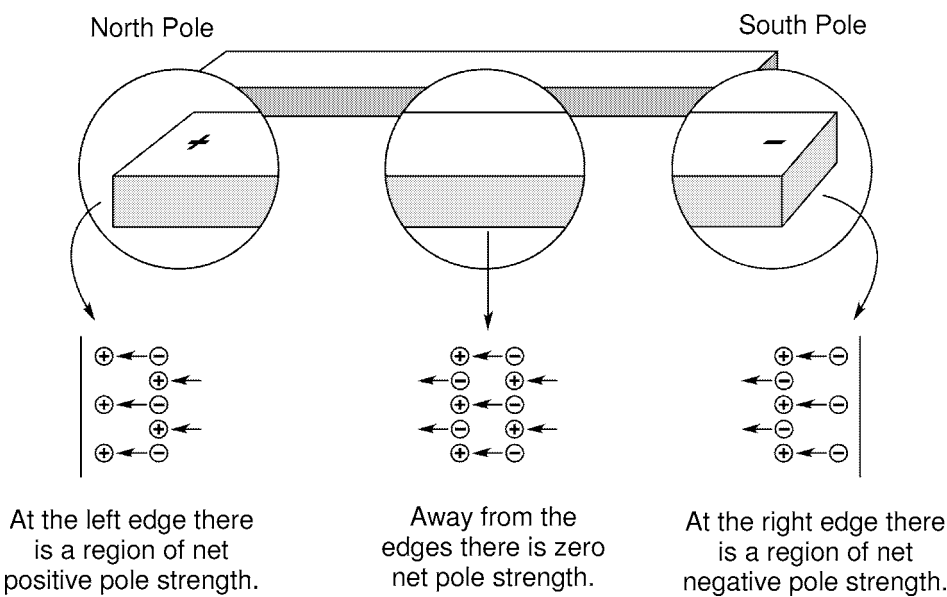
Figure 2.5b A bar magnet can be approximated as a bar-shaped volume of constant permanent-magnet dipole density.
