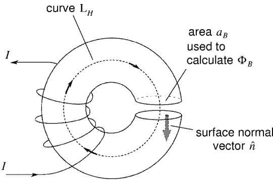
Figure 4.3 Curve L_H is used to define the magnetomotive force \mathcal{F} .
