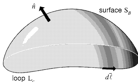
Figure 4.8 Loop L_c is the edge of (unclosed) surface S_B .
