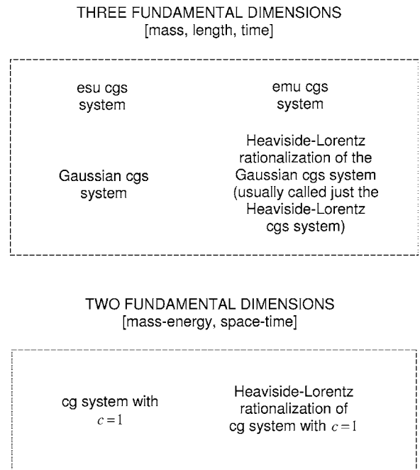
Figure 3.1 Here are six electromagnetic systems which do not recognize charge as a fundamental dimension.
