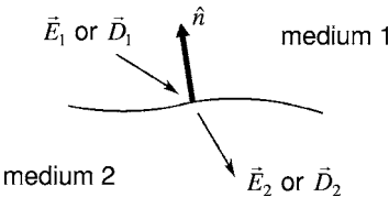
Figure 4.1 The tangential component of the E field is always continuous across the surface between medium 1 and medium 2 and the normal component of the D field may be discontinuous.
