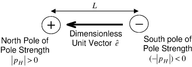
Figure 2.5a The permanent-magnet dipole moment at a point is defined to be \vec{m}_H = [\lim_{\substack{|p_H| \rightarrow \infty \\ L \rightarrow 0}} (|p_H| \cdot L)] \hat{e} .
