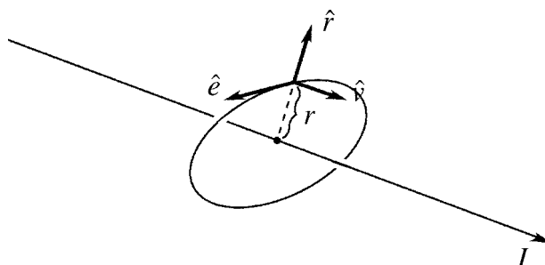
Figure 2.4 Unit-length vectors \hat{e} , \hat{r} , and \hat{\nu} are used to specify the magnetic field generated by current I .
