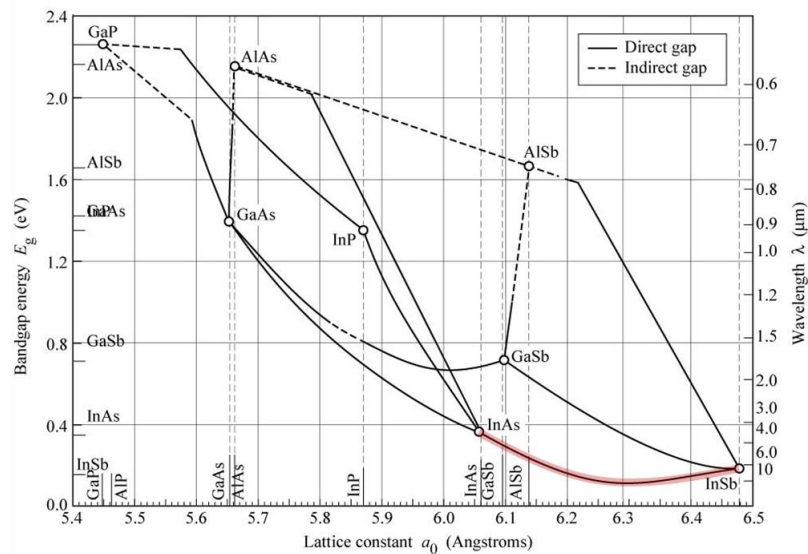
Figure 3.1 – Room temperature band gap energy versus lattice constant of III – V semiconductors, with the InAsSb alloy highlighted (red line) [21]. The minimum band gap of 0.1 eV is achieved for the alloy composition of Sb = 60 %.
