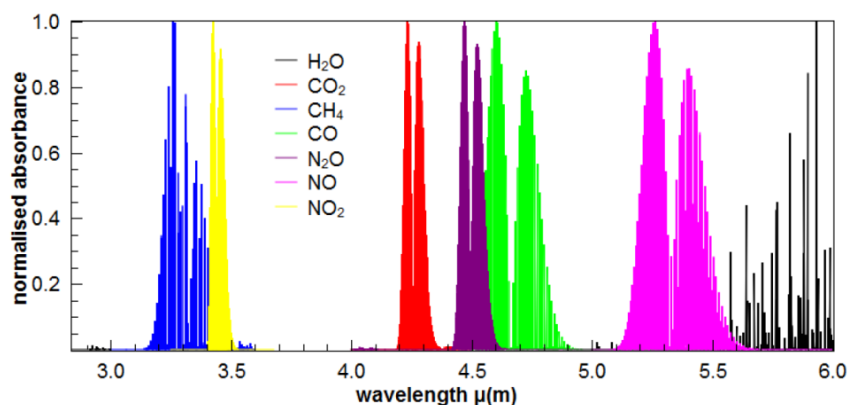
Figure 1.1 – Absorption signatures of gases in the mid-infrared (MIR) spectral region [1], including methane (CH 4 ) at 3.3 \mu\text{m} , carbon dioxide (CO 2 ) at 4.2 \mu\text{m} and carbon monoxide (CO) at 4.6 \mu\text{m} .
